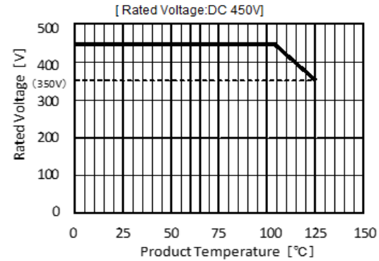
Fig:Derating
