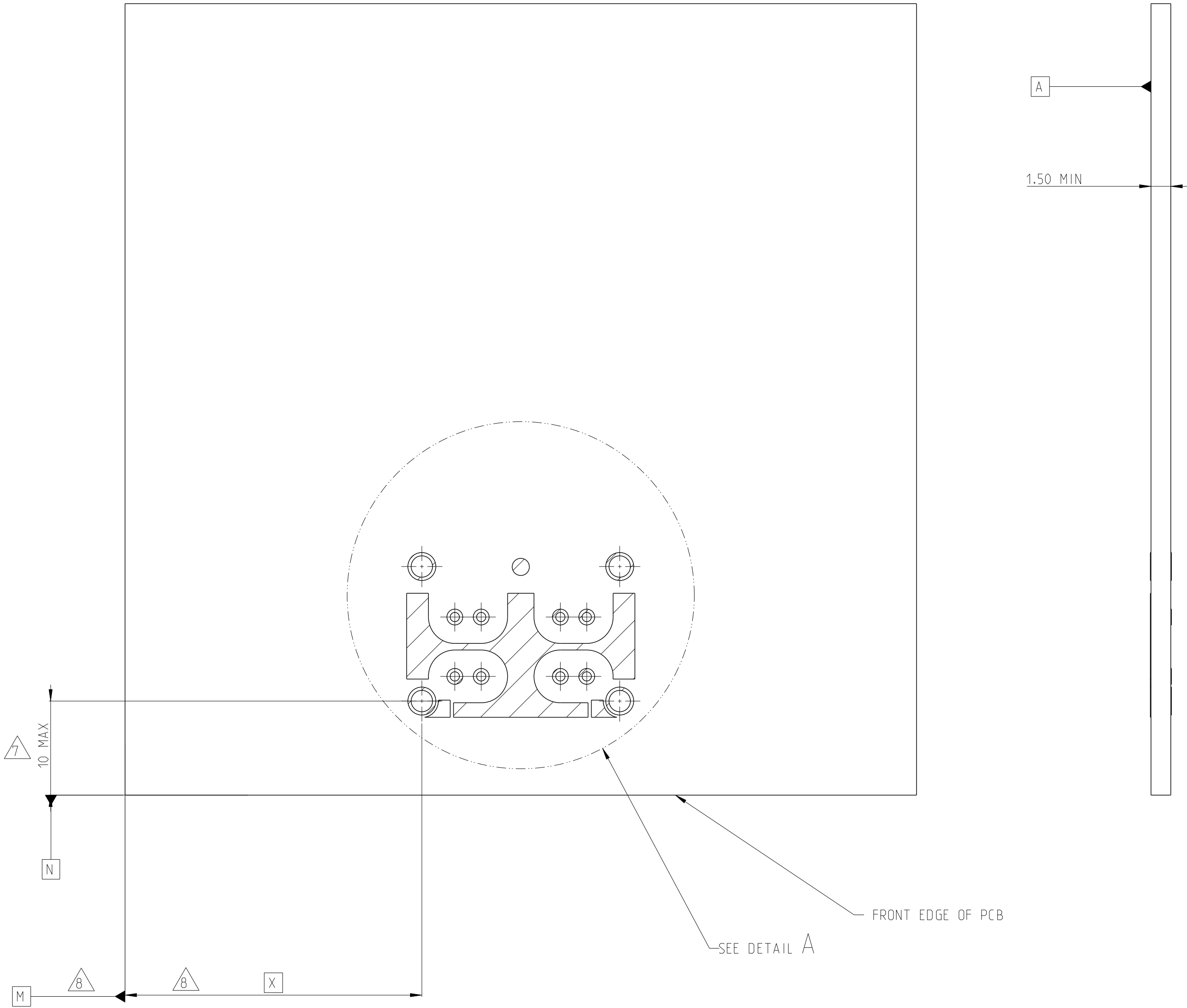
RECOMMENDED PDB FOOTPRINT
