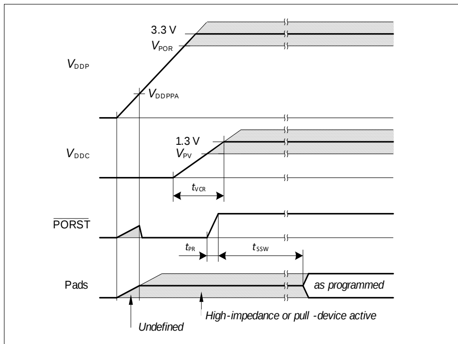
Figure 26 Power-Up Behavior
